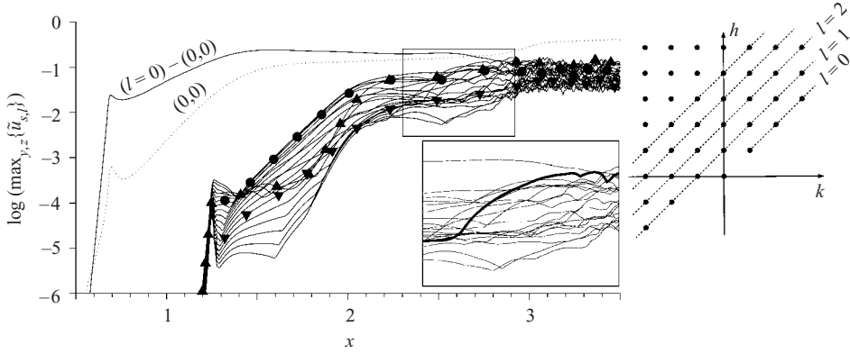
FIGURE 18. Downstream t -modal amplitude development for case WAVE + B in the moving system: single crossflow wave plus periodic background pulses. Frequencies from \beta_m = 0 to \beta_m = 238 , \Delta\beta_m = 14 , are shown. The curve denoted by (l=0) - (0,0) represents the unsteady primary saturated state that is steady ( \beta_m = 0 ) in the moving system. \blacktriangle , \beta_m = 14 ; \bullet , 98; \blacktriangledown , 210. The insert shows a close-up with the frequency \beta_m = 42 emphasized. The sketch on the right-hand side illustrates the coherence of (t-z) -modal and t -modal decomposition in the fixed and the moving system, respectively.
